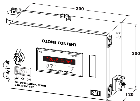
dimensional outline
